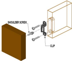
Single Clip
