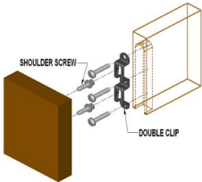
Double Clip
